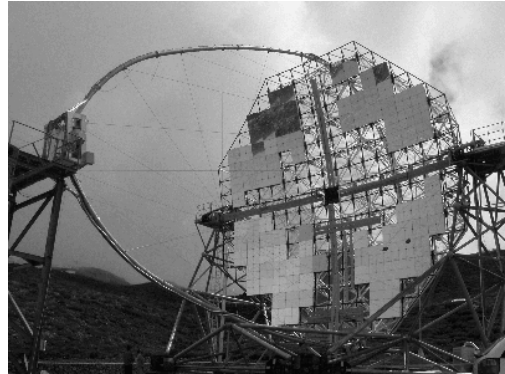
Figure 1. View of the MAGIC telescope just after the camera installation Dec 2002, with 40% of the mirrors installed
