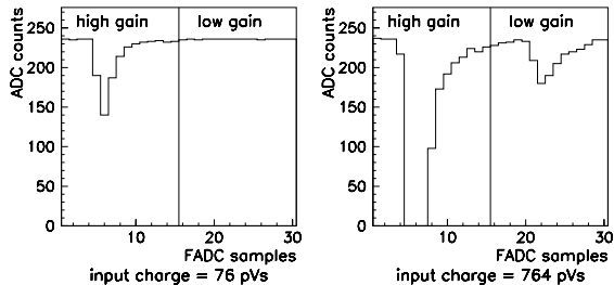
Figure 2. Two test pulses with different input charge read by the MAGIC DAQ. When a large signal make the high gain branch saturated, the low gain side appear 50 ns later (right plot).
